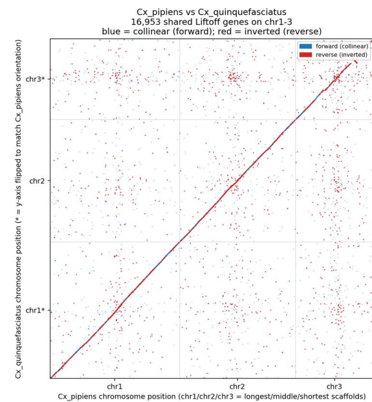
(F) pipiens vs quinquefasciatus
