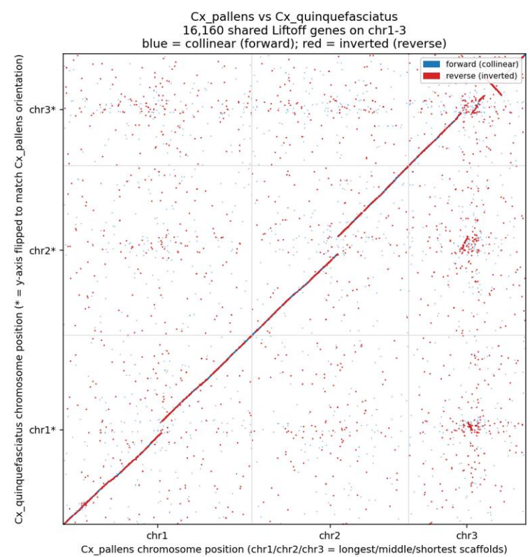
(E) pallens vs quinquefasciatus
